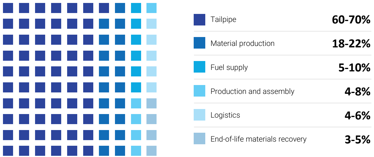
Percentage of total current lifecycle emissions of internal combustion engine vehicles 1
