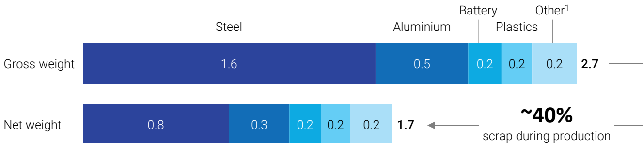
Material inputs for passenger cars, tons per average BEV
